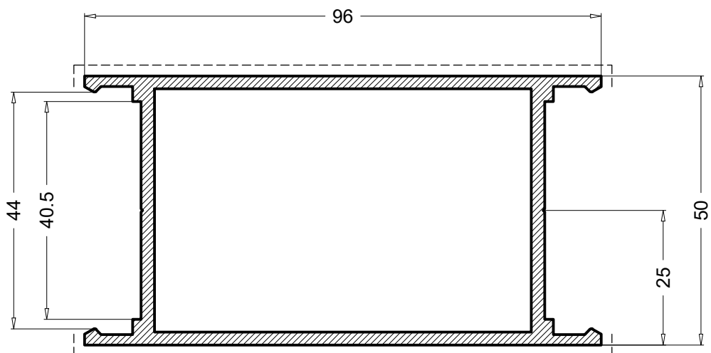
OE80130 1.871 Kg/m
