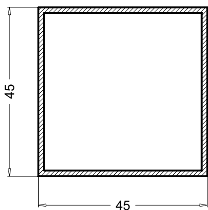
TQ45451.5 0.704 Kg/m
