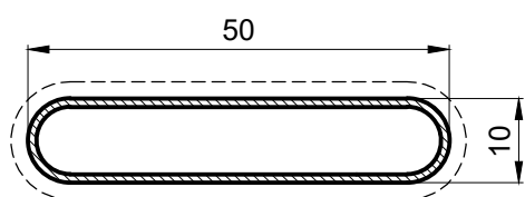
PS12593 0.7 Kg/m
