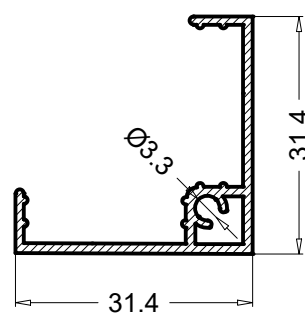
OE80118 0.324 Kg/m
